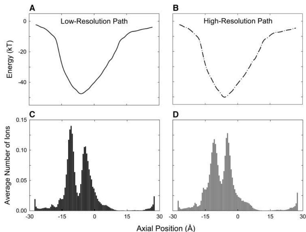
FIGURE 10 Energy profiles and dwell histograms obtained from the models based on the pathways created from the low-resolution (A and C) and high-resolution x-ray structures (B and D).
