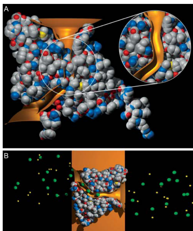
FIGURE 1 The shape of the model channel and Brownian dynamics simulation system. The atomic detail of the crystal structure of the E. coli channel, EcCIC, taken from Dutzler et al. (2002) (A) and our open model of the channel (inset) are shown with the front half of the atoms removed to reveal the pore. The surface of the open pore in gold is superimposed on each diagram. (B) A cylindrical reservoir containing a fixed number of \text{Na}^+ (shown in yellow) and \text{Cl}^- (green) is attached at each end of the channel for Brownian dynamics simulation. The channel protein is imbedded in a low dielectric region representing the membrane (gold).
