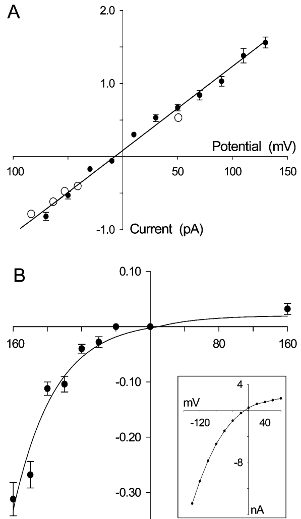
FIGURE 5 The current-voltage relationships of CIC-0 (A) and CIC-1 (B). The current measured at various applied potentials is obtained with symmetrical solutions of 150 mM in both reservoirs. In this and all subsequent figures, unless stated otherwise, a data point ( solid circle ) represents the average of 24–48 sets of simulations, each set lasting 4 \times 10^6 time steps (or 0.4 \mu\text{s} ). Error bars in this and following figures have a length of \text{mean} \pm \text{SE} of 1 and are not shown when they are smaller than the data points. Superimposed on the simulated data in A are the experimental measurements obtained by Miller (1982), shown in open circles. The whole-cell current-voltage relationship illustrated in the inset of B is reproduced from Bennetts et al. (2001).
